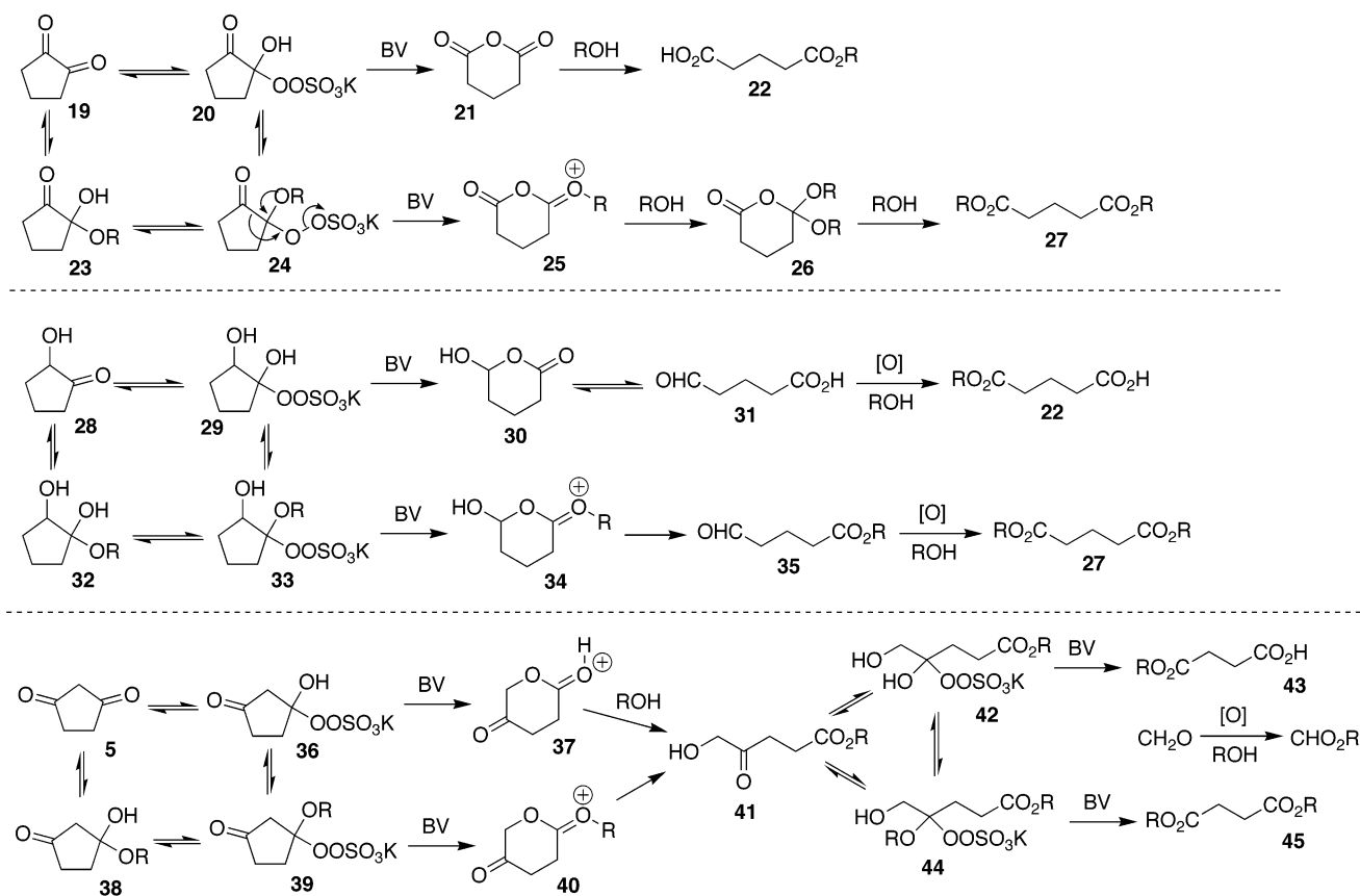
SCHEME 2. Probable Mechanistic Routes for the Oxidative Cleavage of \alpha - and \beta -Diones and \alpha -Hydroxyketones
